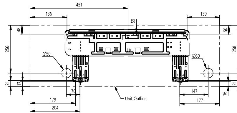
Fixing the installation plate, drilling hole
