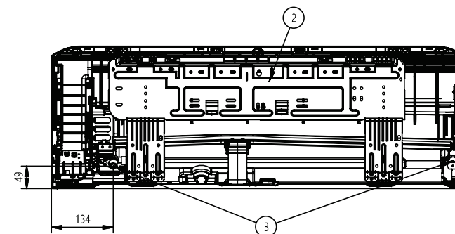
Fixing the installation plate, drilling hole
