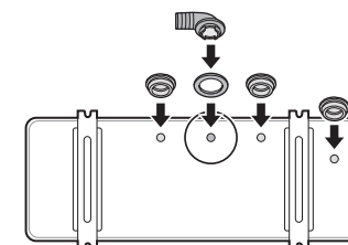
Drain Plug
