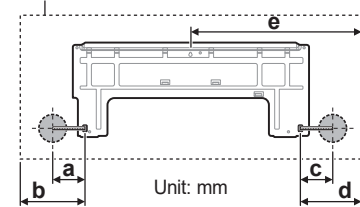
Framework of Indoor Unit
