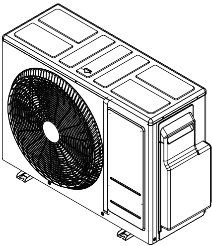
3D VIEW
